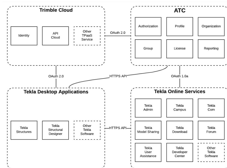
Image 1. Tekla Online architecture
