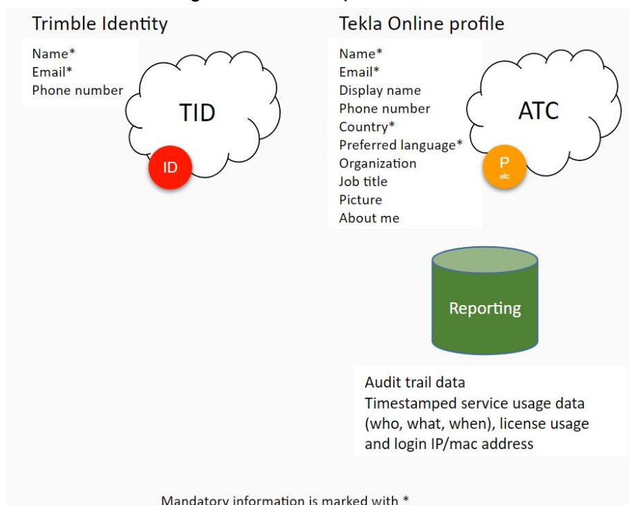
Image 2. Personal data in Tekla Online licensing solution
